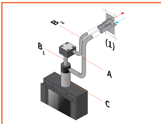
Figure 3.5 - (Partial) concentric flue configuration with horizontal terminal in the same area
