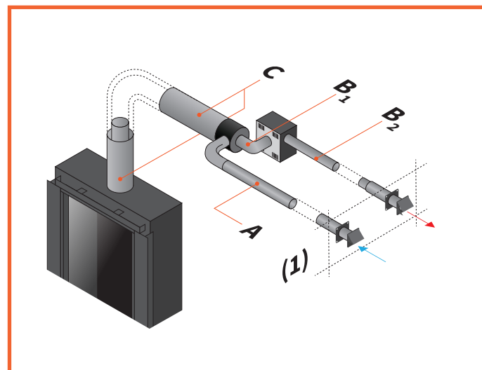
Figure 3.8 - (Partial) concentric flue configuration with horizontal terminal in the same area (II)
