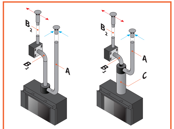
Figure 1.6 - Vertical terminals
