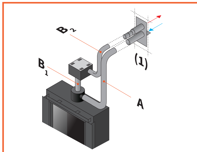
Figure 3.2 - Adapter directly on the fireplace and with horizontal terminal in the same area
