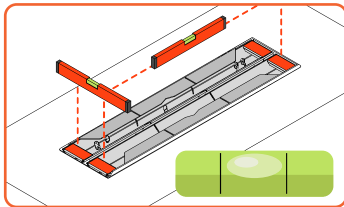
Figure 5.1 | Make sure the burner is level
