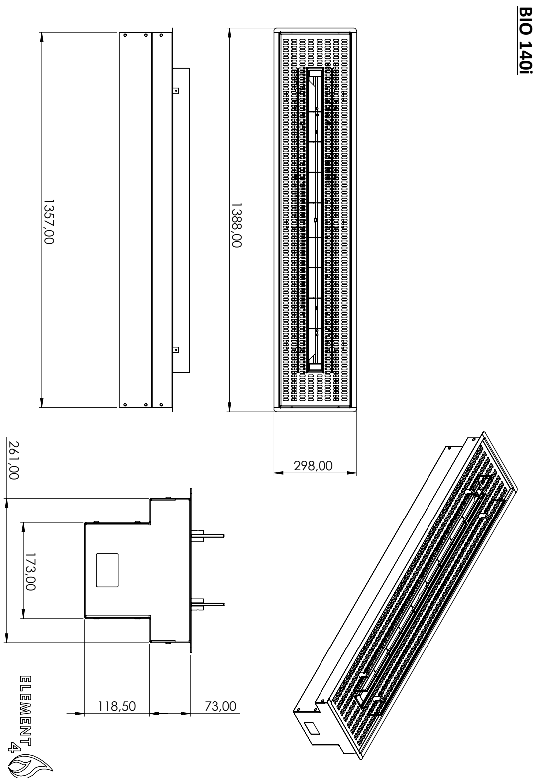
Figure E.A | Technical drawing of Bio 140i
