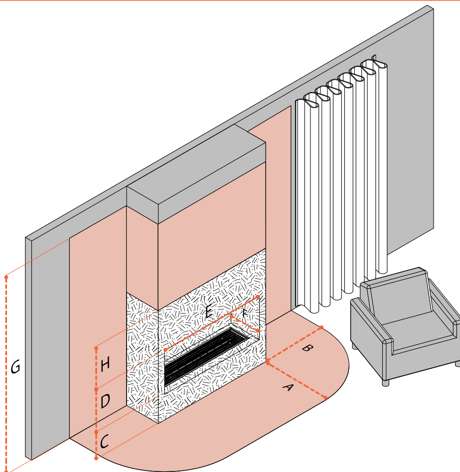
Figure 5.2 | Requirements installation location
