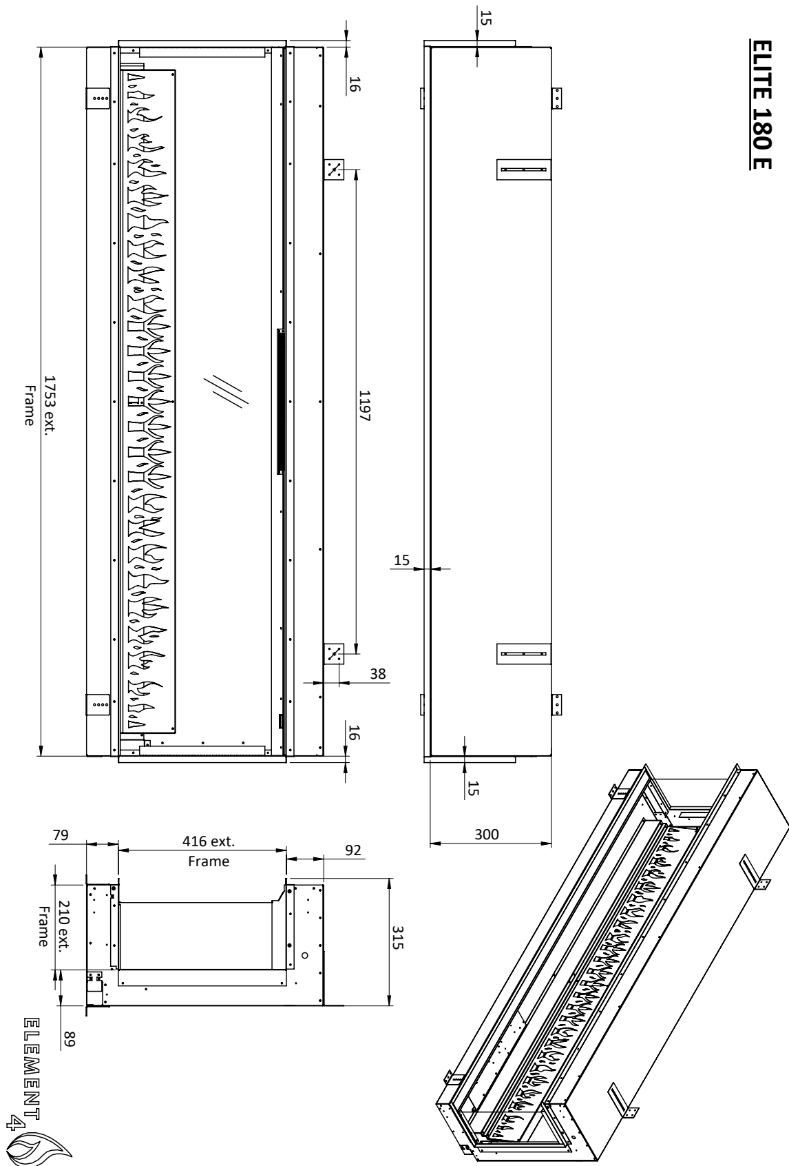
Figure.B.J | Elite 180-E Supreme dimensions
