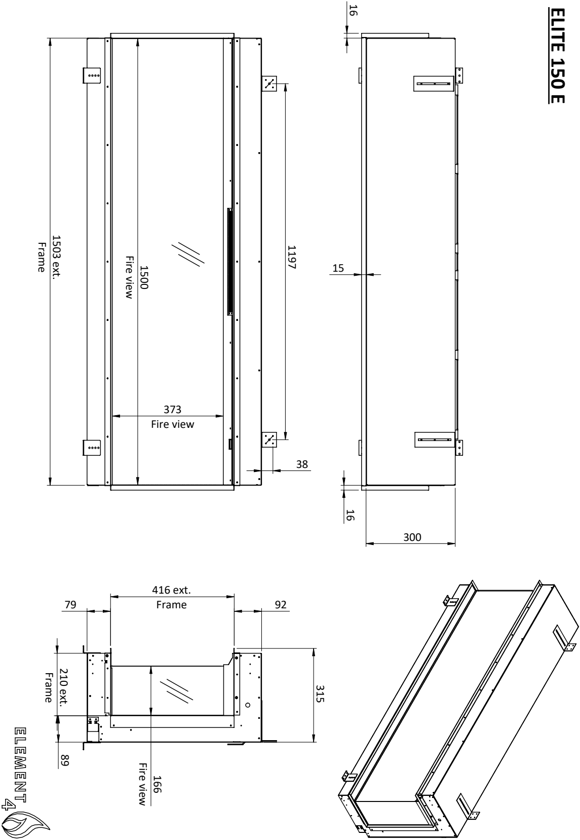
Figure.B.I | Elite 150-E Supreme dimensions
