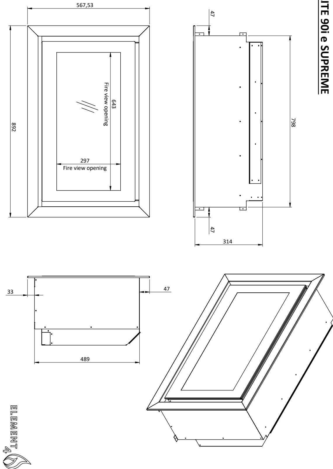
Figure.B.D | Elite 90I-E Supreme dimensions
