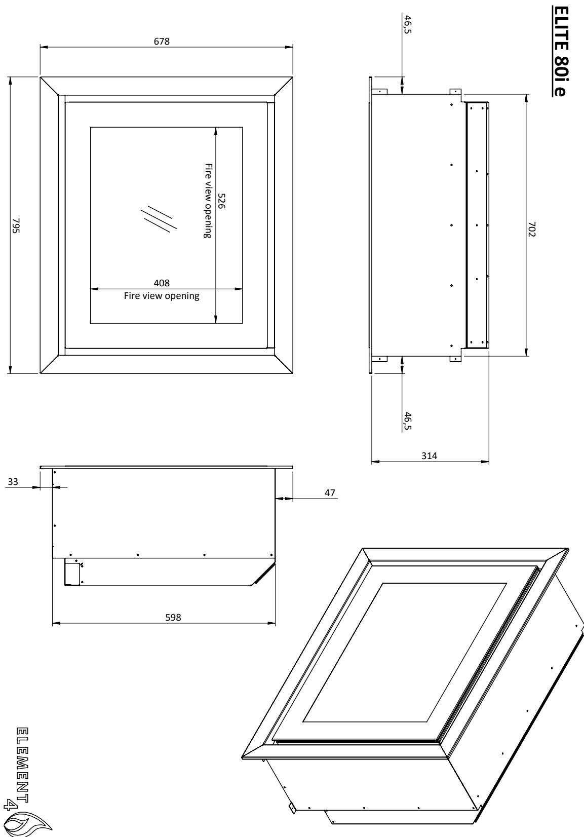
Figure.B.C | Elite 80i-E Supreme dimensions
